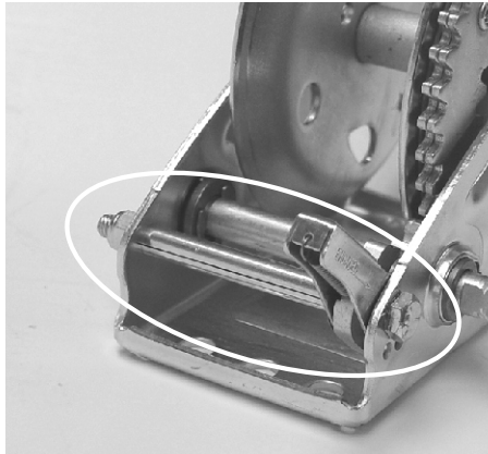
RATCHET STOP MECHANISM
